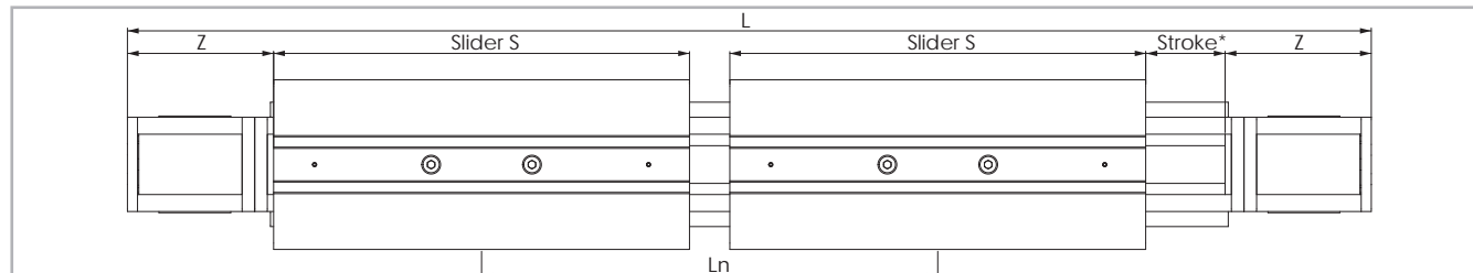
* The length of the safety stroke is provided on request according to the customer's specific requirements. Fig. 56
